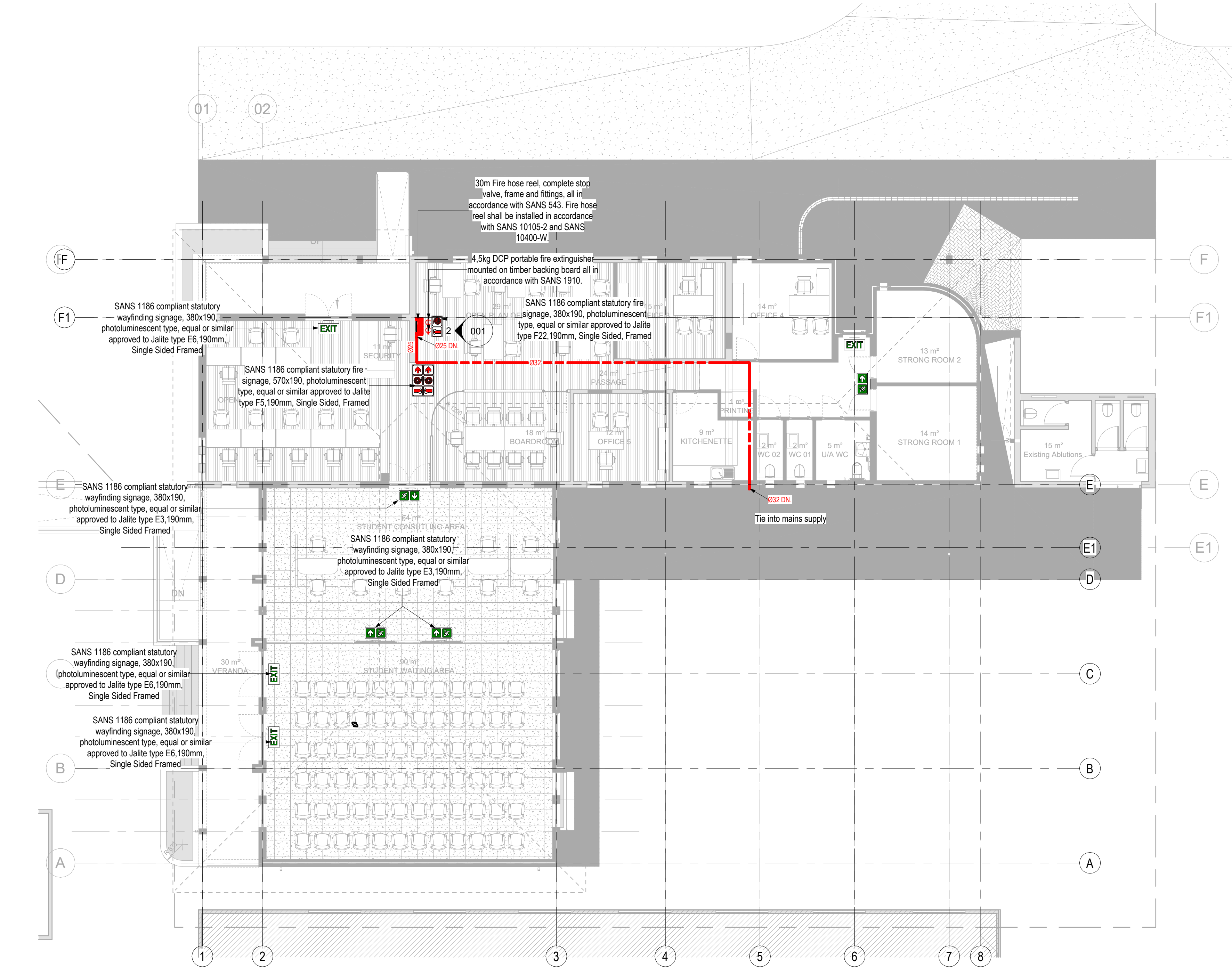
1 GROUND FLOOR 1 : 100
